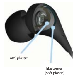
Hybrid material driver housing
