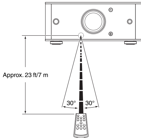
[Horizontal installation]
